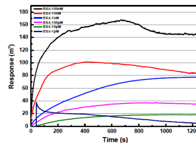
Sensogram corresponding to various concentrations of BSA
