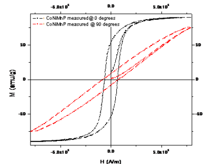
Hysteresis loops anisotropic CoNiMnP thick layers
