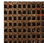
Electroplated CoNiMnP permanent magnets in SU8 pattern, optical microscopy, x 50
