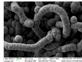
Positive electrode -polypyrrole deposited by cyclic voltammetry on CNTs
